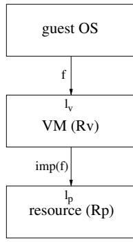
Figure 1. Virtual Machines
