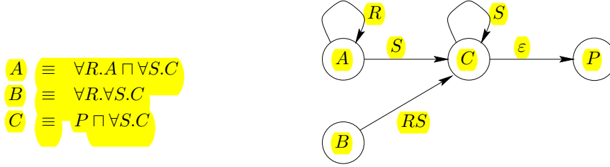
Fig. 2.7. A TBox and the corresponding automaton.
