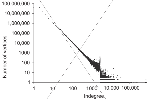
Figure 8.24: The distribution of indegrees of a WebBase crawl. From [Donato et al., 2007].
