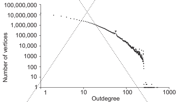
Figure 8.25: The distribution of outdegrees of a WebBase crawl. From [Donato et al., 2007].
