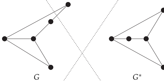
Figure 2.9: Two nonisomorphic graphs with the same ordered degree sequence.
