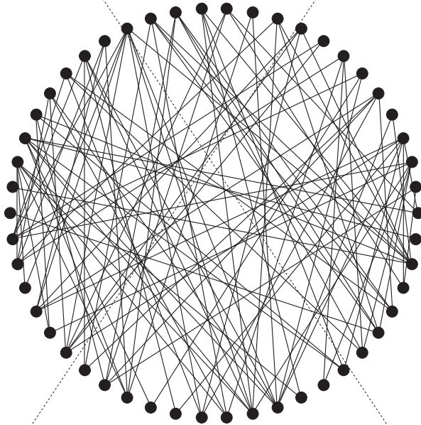
Figure 2.14: A random graph with 50 vertices and 103 edges. The circular embedding allows to draw each edge as a straight line that remains (reasonably) visible.
