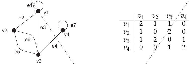
Figure 2.6: A graph with its associated adjacency matrix.
