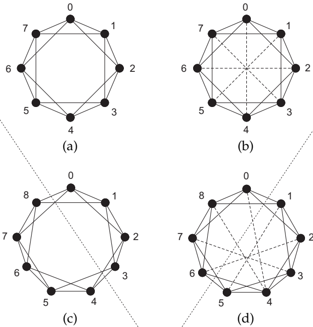
Figure 2.11: Various Harary graphs: (a) H_{4,8} , (b) H_{5,8} , (c) H_{4,9} , and (d) H_{5,9} . Dashed edges are the ones added to obtain H_{5,8} from H_{4,8} , and H_{5,9} from H_{4,9} , respectively.
