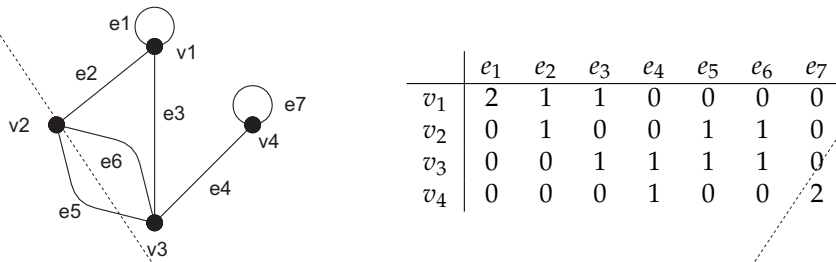
Figure 2.7: A graph with its associated incidence matrix.
