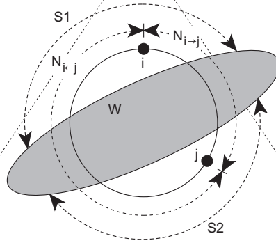
Figure 2.12: Illustration that |W \cap N_{i \rightarrow j}| < k/2 or |W \cap N_{i \leftarrow j}| < k/2 .
