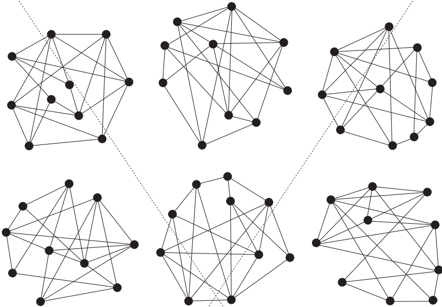
Figure 2.8: Six different drawings of graphs with the same representation, that is, isomorphic graphs.
