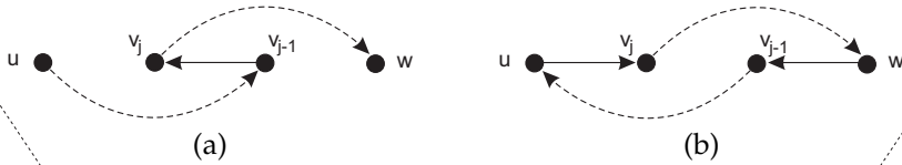
Figure 4.7: (a) A Hamilton path in G , and (b) the constructed Hamilton cycle in G .
