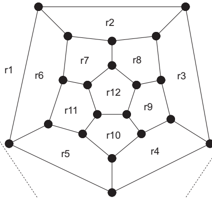
Figure 2.17: A plane graph with 12 regions.
