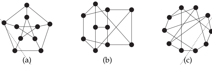
Figure 2.13: Three different drawings of the Petersen graph.
