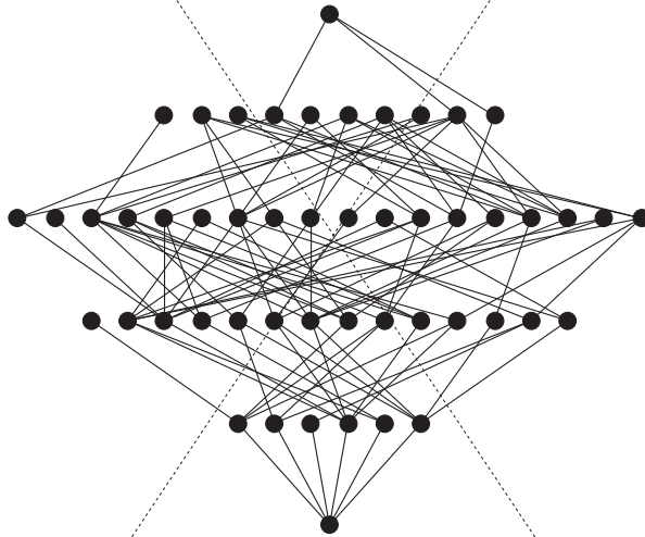
Figure 2.15: A ranked embedding of the graph from Figure 2.14.
