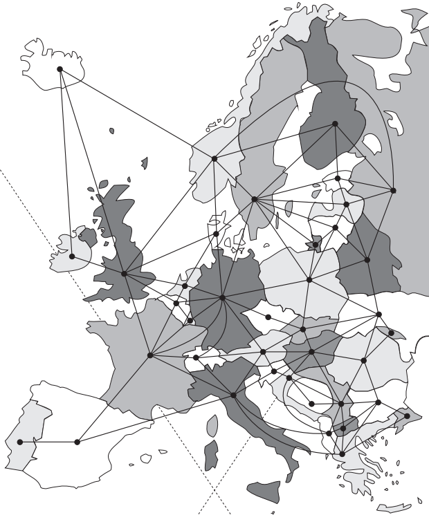
Figure 3.6: A map of Europe and its corresponding representation by a planar graph, along with a four-coloring of the vertices.
