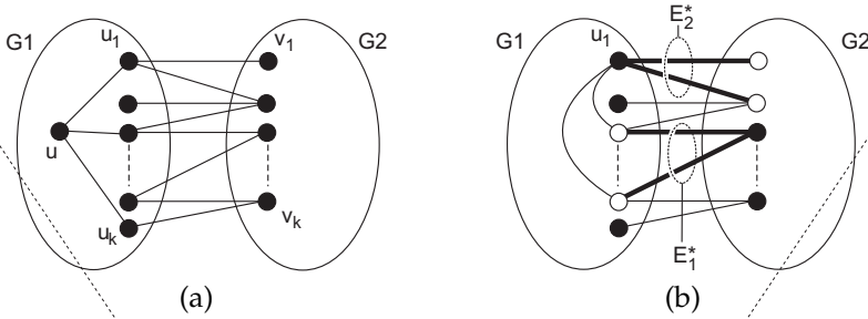
Figure 2.10: The two scenarios for the proof of Theorem 2.4.
