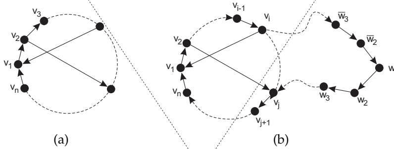
Figure 3.3: The construction of a strongly connected orientation.
