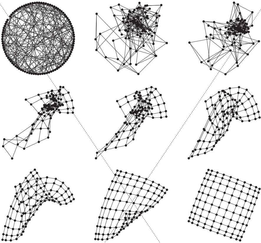
Figure 2.16: The evolution of applying a spring embedding to a graph.
