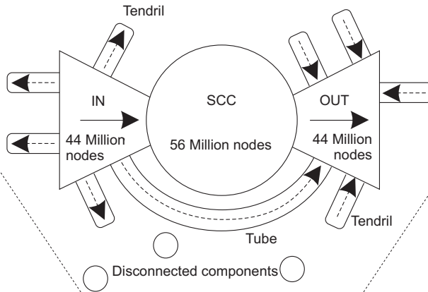
Figure 8.22: The macroscopic structure of the Web from [Broder et al., 2000].
