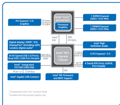
Intel® H61 Express Chipset Platform Block Diagram
