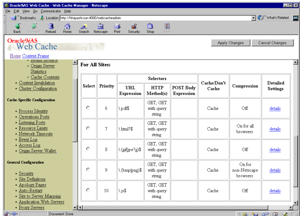
Figure 7-2 Default Global Caching Rules
