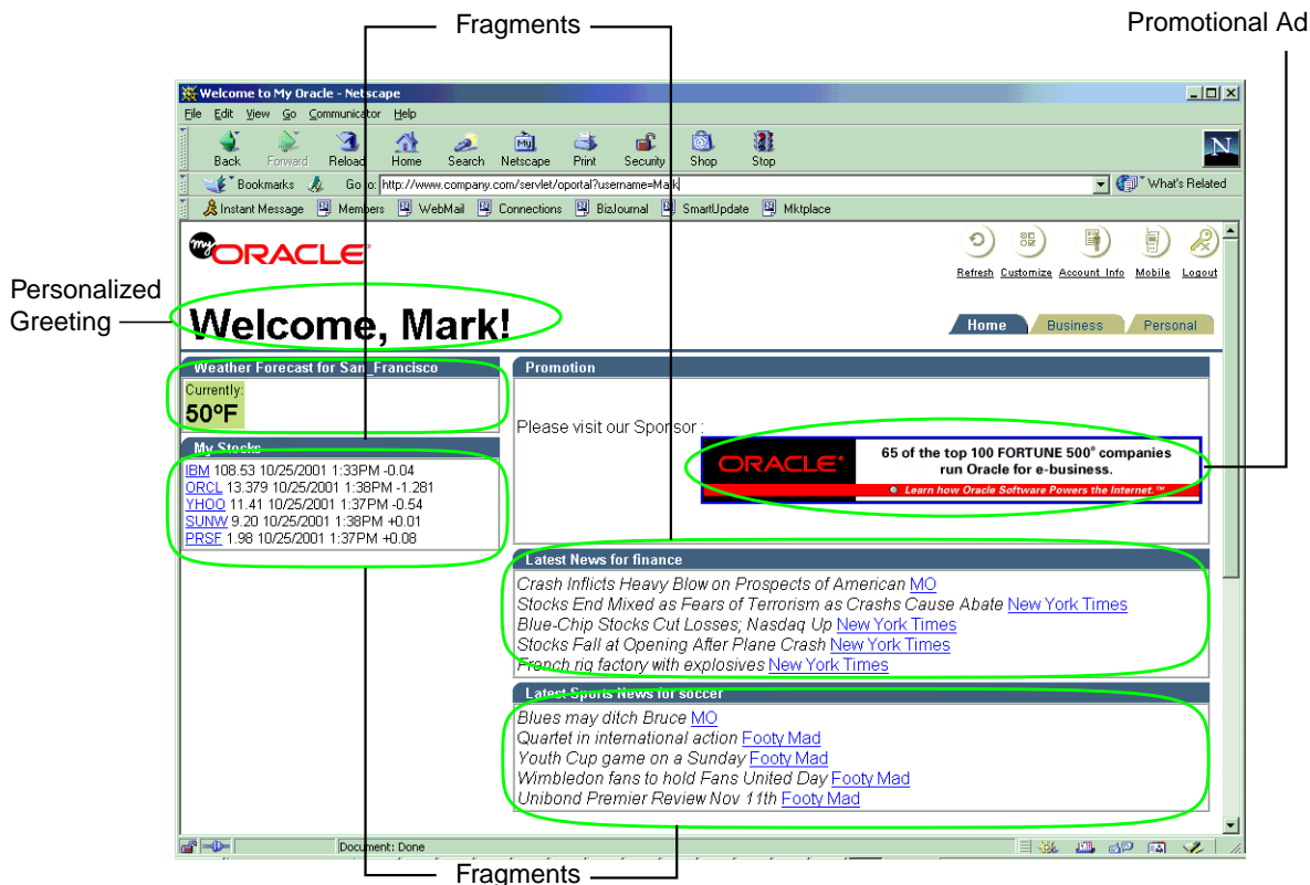
Figure 7-8 Portal Site Page
