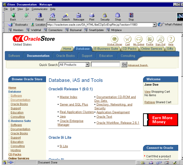
Figure 2–6 Session-Encoded URLs
