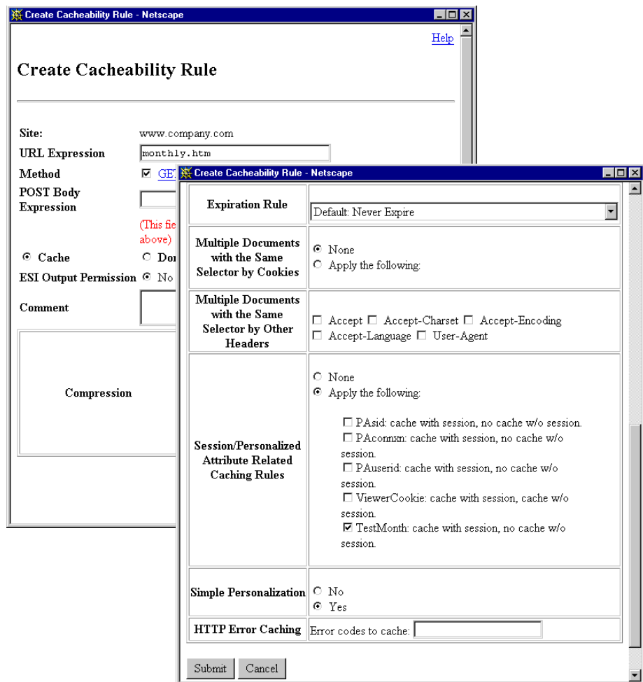
Figure 7-6 Create Cacheability Rule Dialog Box
