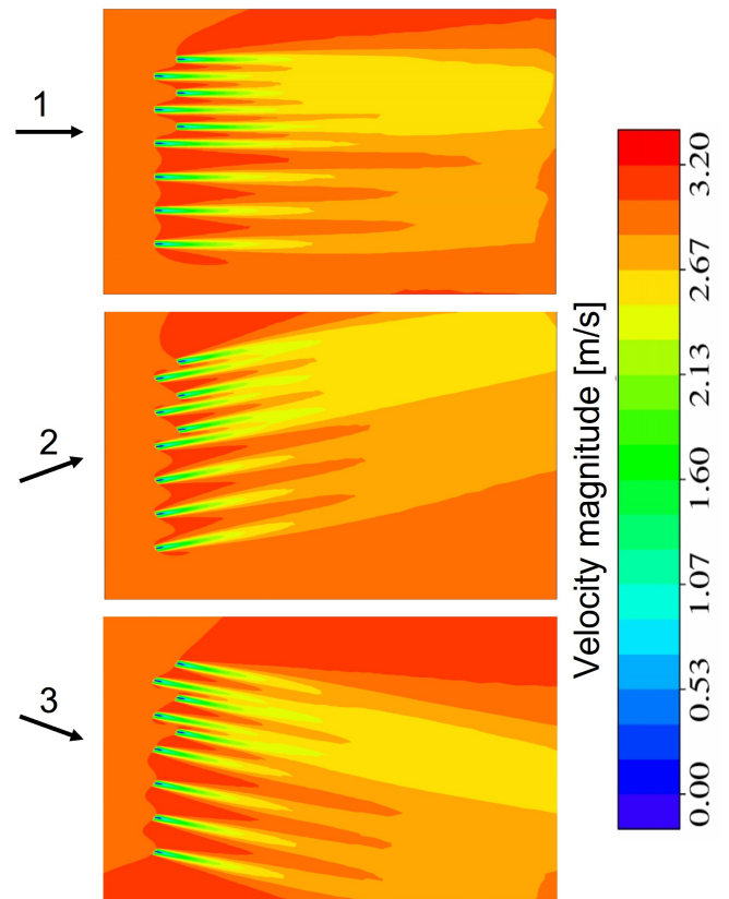
Fig. 10. grid_2 flow field of direction 1, 2, and 3. The flow fields are plotted on the horizontal middle plane.
