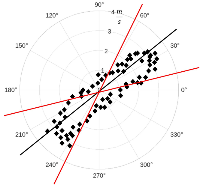
Fig. 6. Qualitative representation of velocity data spread in a site characterized by an elliptical polar graph. We can identify a prevalent direction (black line), and around it consider a tolerance range of directions bounded by the red lines, with suitable velocity for energy exploitation.
