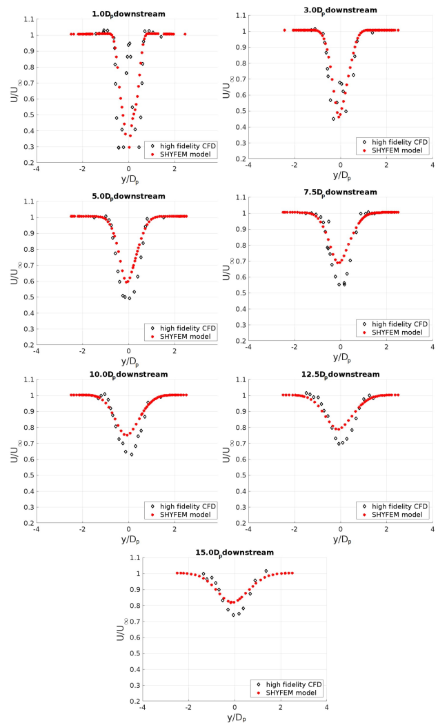
Fig. 3. Wake velocity profiles relative to the horizontal middle plane for a 10 m diameter turbine: comparison between the SHYFEM model (red asterisks) at the optimal TSR i.e. 3, and the high fidelity CFD of [11] (black diamonds) at the optimal TSR i.e. 3.64.
