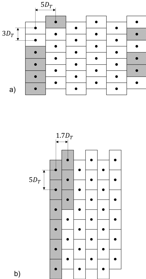
Fig. 8. a) grid_1 conventional staggered grid, and b) grid_2 site-adapted staggered grid. The shaded rectangles represent locations occupied by the 9 turbines of the cluster we wanted to optimize.
