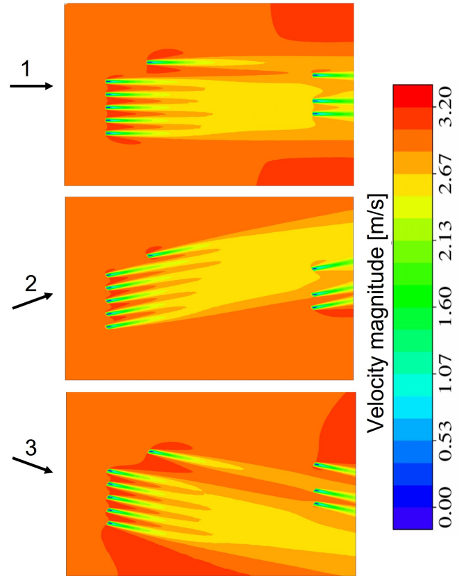
Fig. 9. grid_1 flow field of direction 1, 2, and 3. The flow fields are plotted on the horizontal middle plane.
