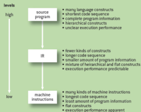
The Different Levels of Program Representations
