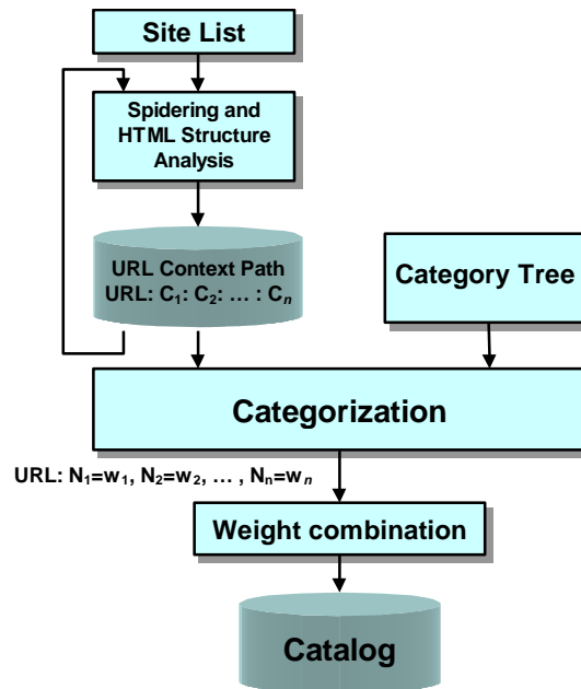
Figure 1: Architecture of Categorization by Context
